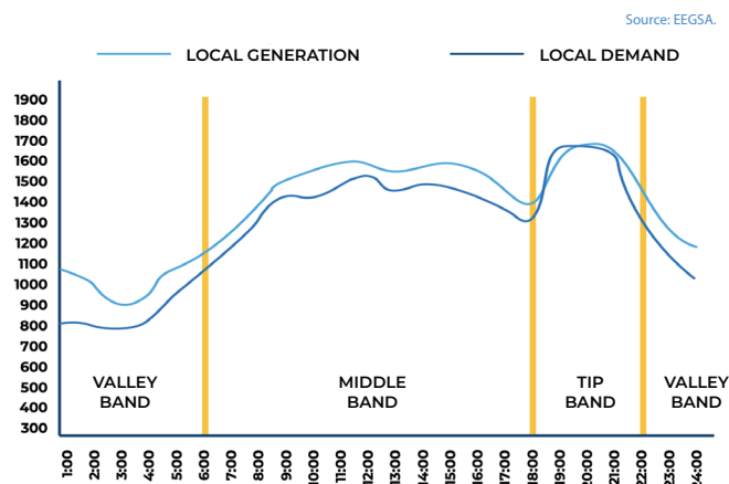
Figure 3: hourly band by demand of SEN.
